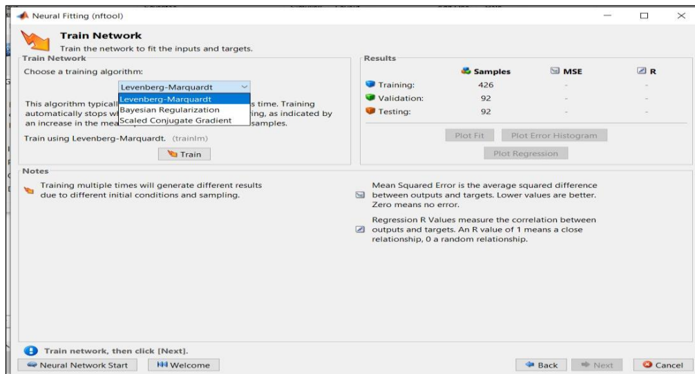
Figure 4- Algorithms
