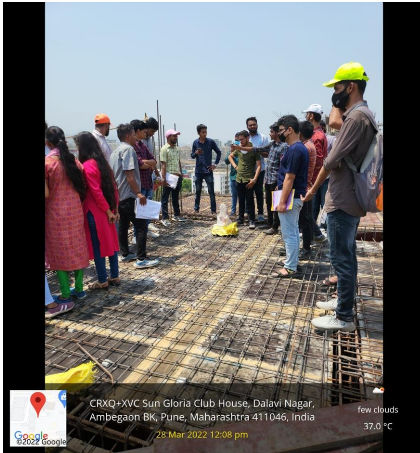
A site visit to study Structural Components with reference to RCC slab
