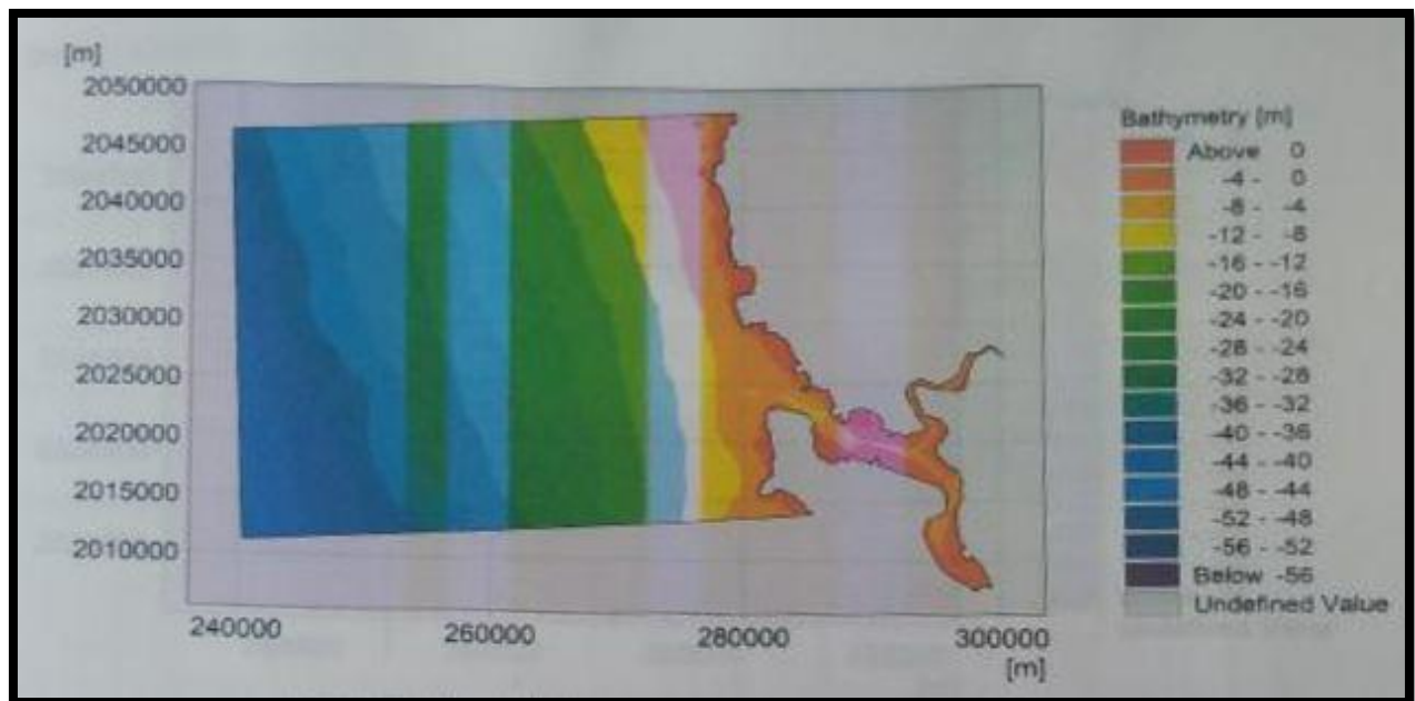
Figure 2-Model Area considered for simulation
