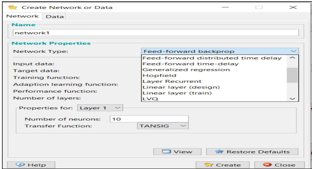
Figure 3- Network Type
