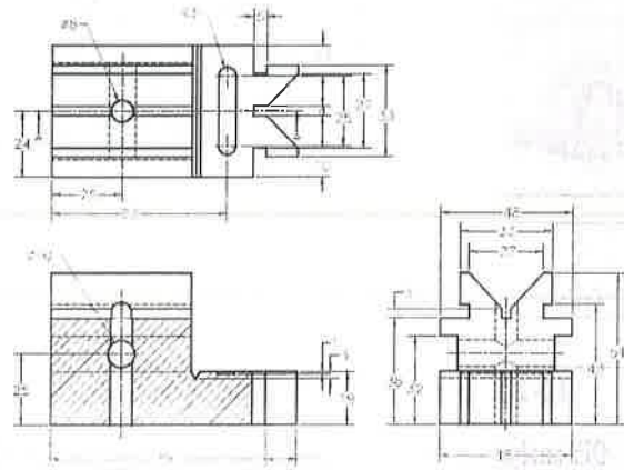
Figure 2 Views and dimensions of the V-Block body.
