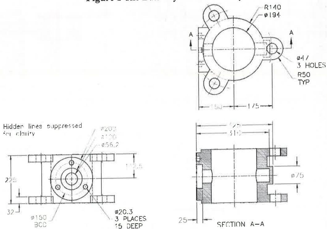
Figure 2 Dimensions of the Body
