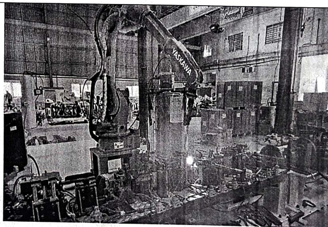
Engineer from PARCRobotics interacting with students of TE explaining the Robot Programming and use of HMI (in the left) and an automation set-up of welding with a robotic system of YASKAWA at the Chakan Plant of PARC Robotics Pvt. Ltd., Pune
