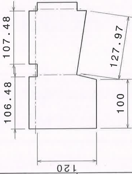
LH--Unfolded view Scale: 1:4
