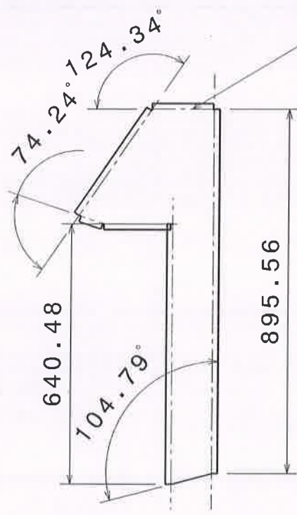
LH Unfolded view Scale: 1:12
